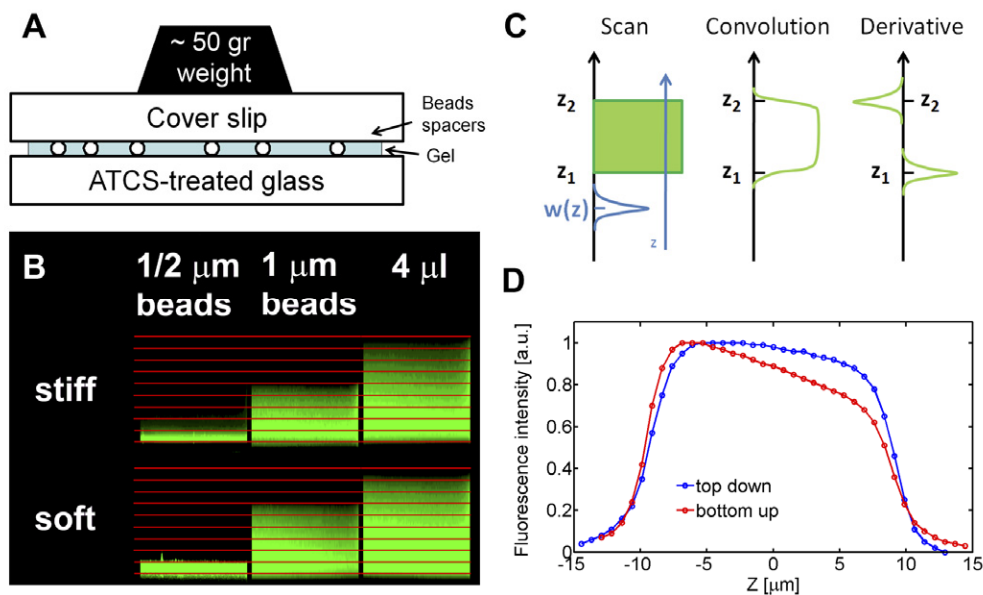
Figure 4. Preparation of thin PA gels. (A) Thin PA gels were polymerized between an ATCS-treated coverslip and a clean coverslip. To control gel thickness, micron-scale bead spacers were included in the gels and pressed between the glass substrates using a weight. (B) Cross-sections of FITC-labeled gels were obtained using a laser scanning confocal microscope. The red grid indicates 2\ \mu\text{m} separation. (C) Gel thickness was evaluated using an edge detector, based on the peak centers of the z -derivative (right). (D) Fluorescence intensity profiles of a thick and soft gel were obtained by top-down and bottom-up laser scanning. Intensity profiles show decreasing intensity towards the gel top surface that becomes more prominent for the latter.
